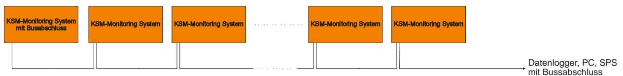
Abb. 4 Verdrahtung RS-485 Bus
